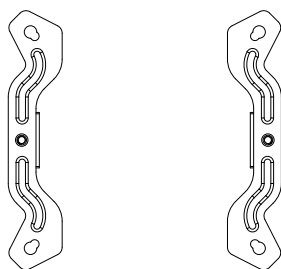
Ⓒ INTEL SOCKET X 2PCS
